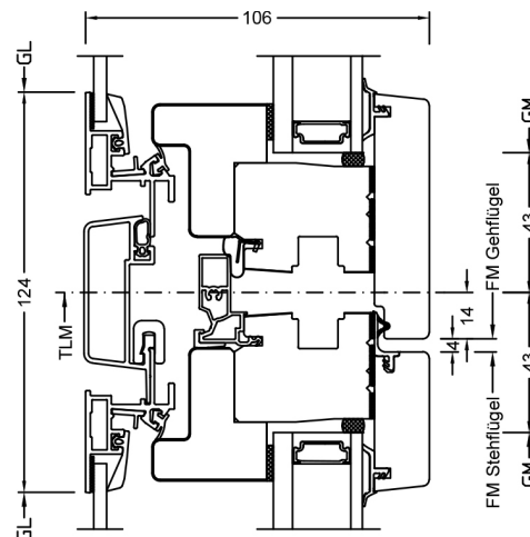
Flying mullion
