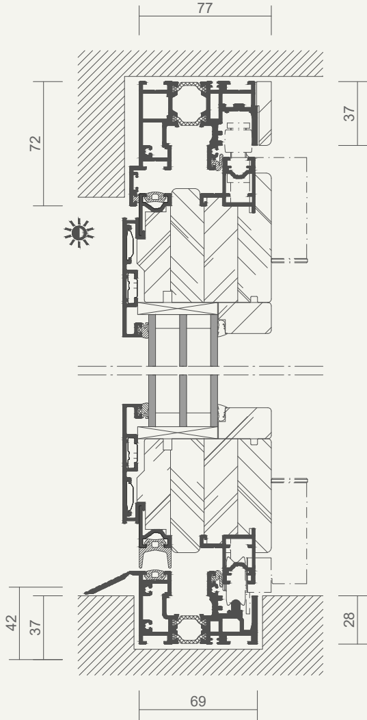
Vertical section
