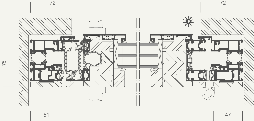
Horizontal section
