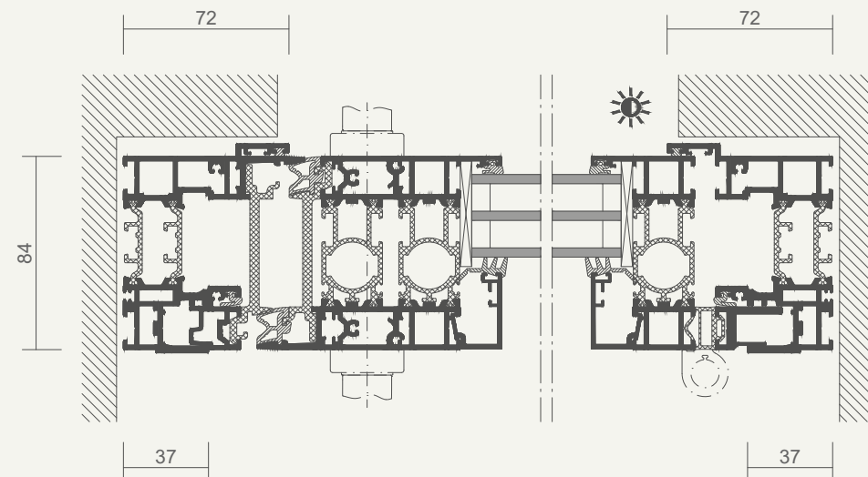
Horizontal section
